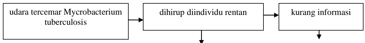
Gambar 2.1 Pathway Tuberculosis Paru
